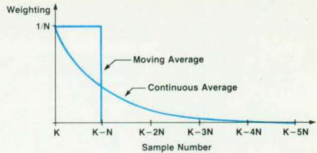
Fig. 8. Graph showing the weighting of samples over time for a moving average and a continuous average.
