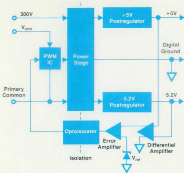
Fig. 3. Pulse width modulation (PWM) voltage control.
