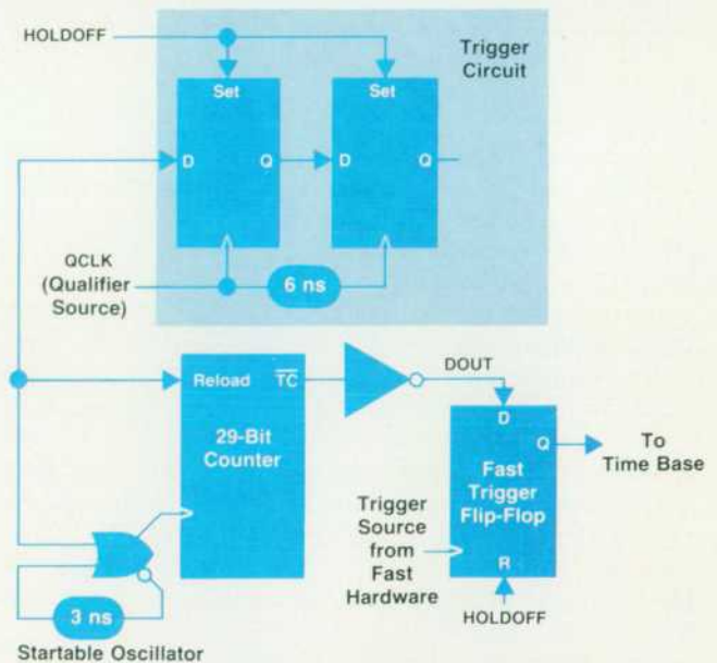
Fig. 8. Block diagram of the HP 54100AD triggering system in Time-Delay mode. The startable oscillator and counter are configured as a timer that is started by a trigger circuit. This allows time to be counted from an edge at QCLK before arming the fast trigger flip-flop.
