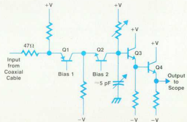
Fig. 3. Simplified schematic of the active network in the HP 54001A Miniature Active Probe.
