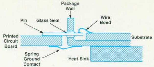
Fig. 7. Cross section of hybrid circuit package assembly.
