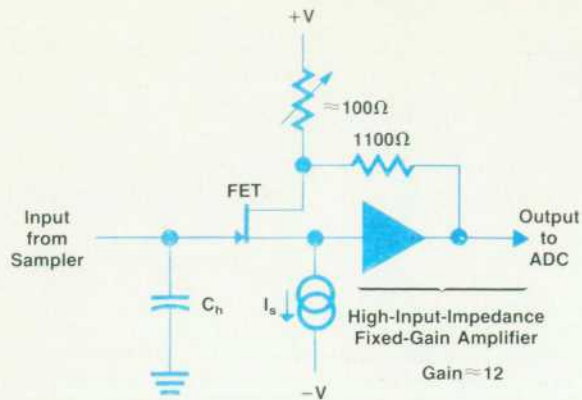
Fig. 12. Simplified postamplifier schematic diagram.
