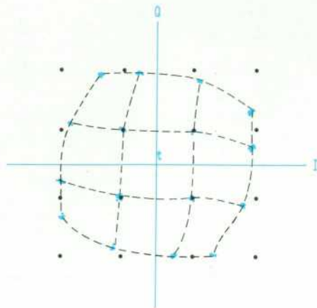
Fig. 8. The nonlinear characteristics of high-power amplifiers are highly visible on displays of digital microwave radio signal states like this constellation diagram. The compression of the amplifier at high amplitudes causes the outermost states to be drawn in. The amplitude dependent phase shifts also cause the outermost states to be rotated. A 16QAM modulation was used for this diagram because the amplitude variations help to excite the nonlinear channel. I•Q Tutor allows varying degrees of nonlinearities to be selected to observe the increase in degradation with increased amplifier drive levels.
