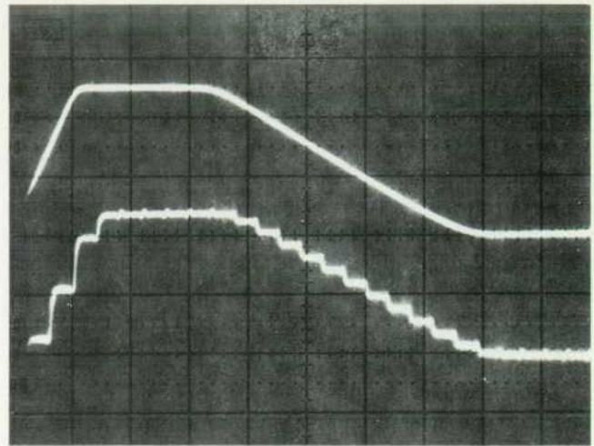
Fig. 13. A ramp-type input to the sampler and the output of the postamplifier held in steps 25\text{ ns} apart.
